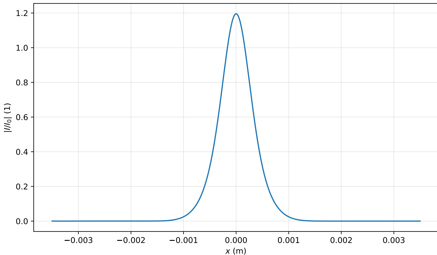
Intensity profile I(x, y = 0, z = 0.955m)/I_0 , P_{in}=0.7P_{cr} , artificial time
